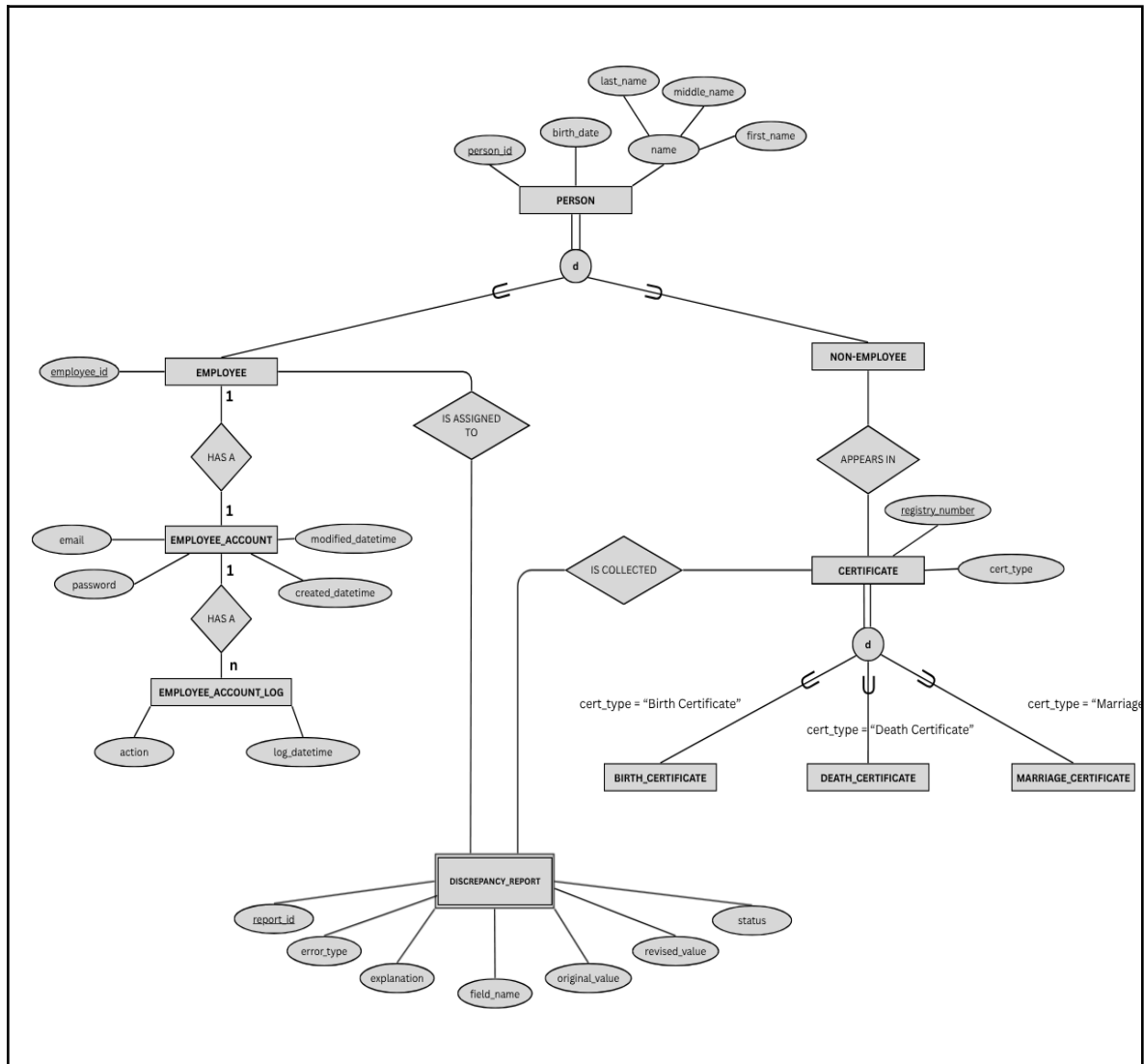
Figure 5.2: Enhanced Entity Relationship Diagram of the Database System
