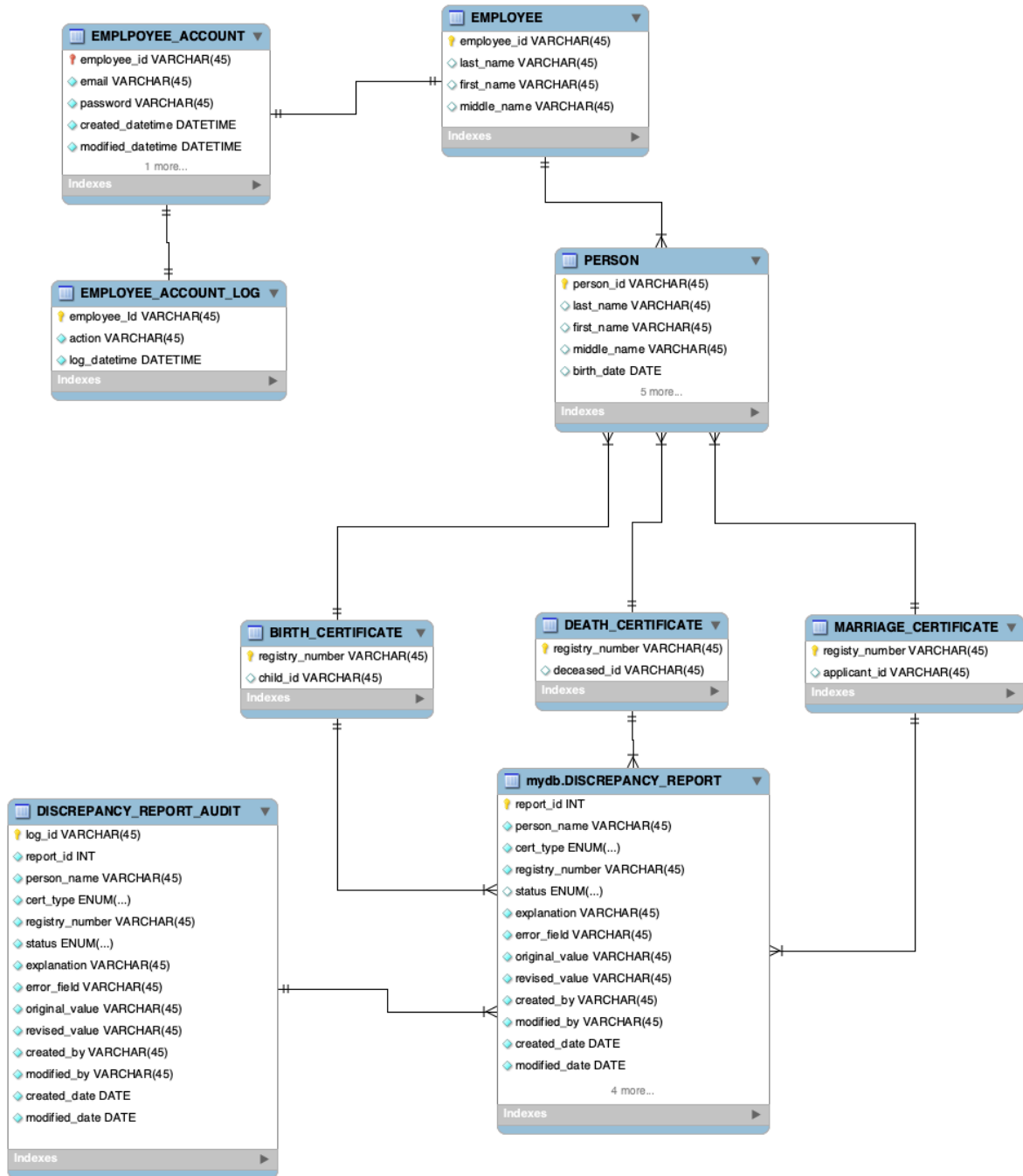
Figure 5.1: Entity Relationship Diagram of the Database System
